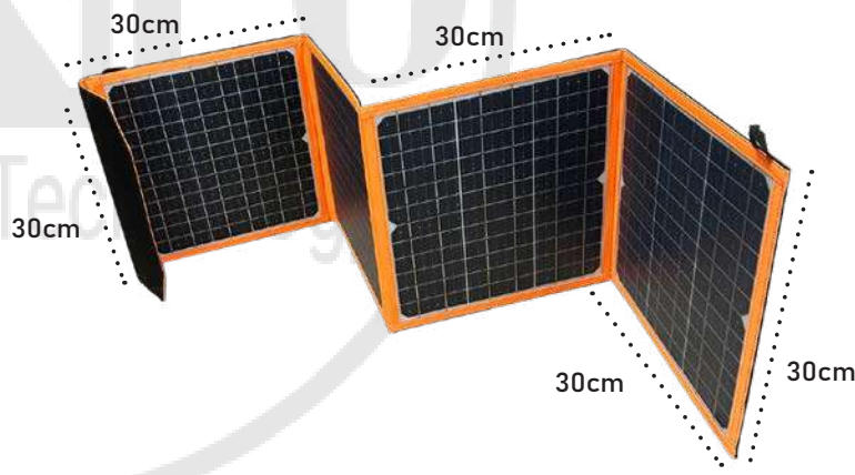
PANEL SOLAR 40W TIPO FOLDER X4
