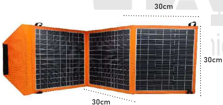
PANEL SOLAR 30W TIPO FOLDER X3
